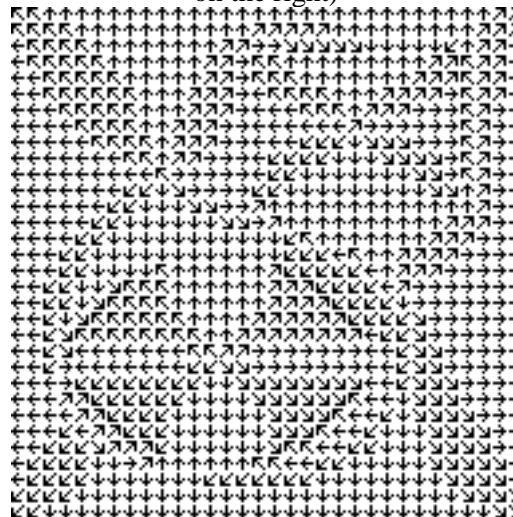
Fig. 2.8 The vector length in the transformed field of test3 (the original image; 4 times of original size on the right)
